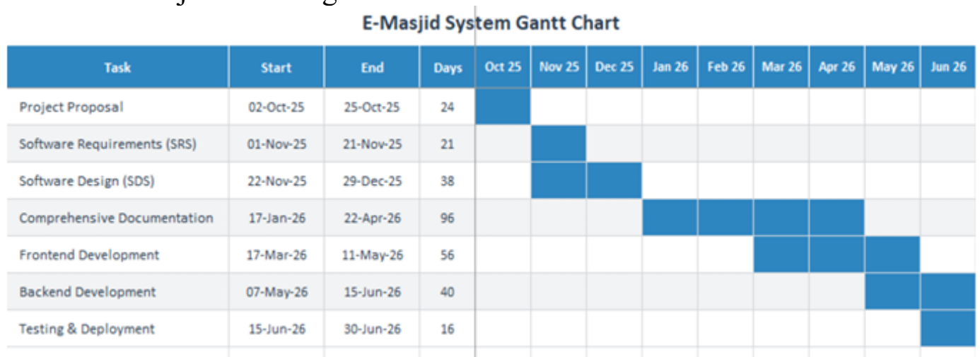
Figure 1 Gantt Chart
