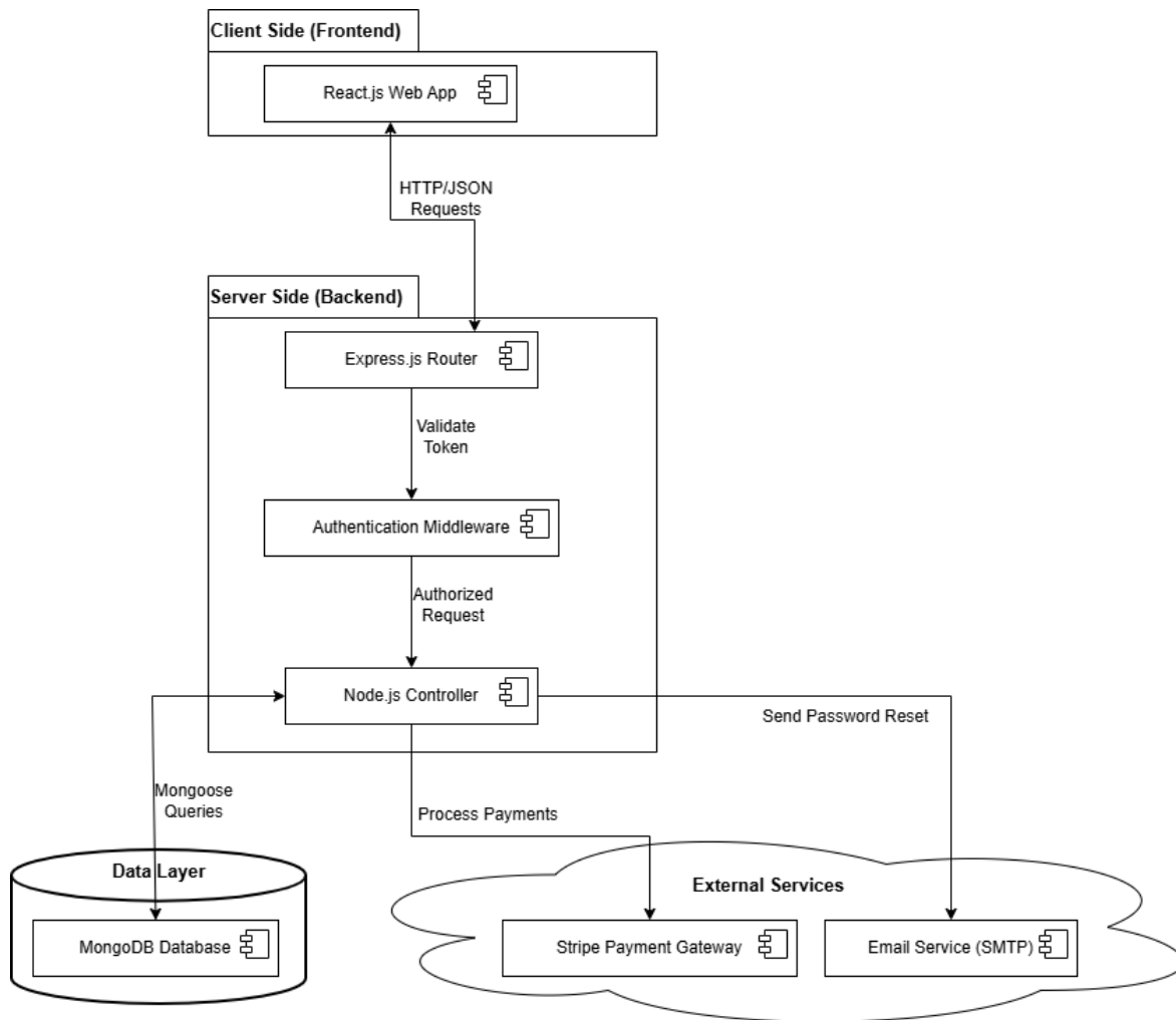
Figure 20 Architectural diagram
