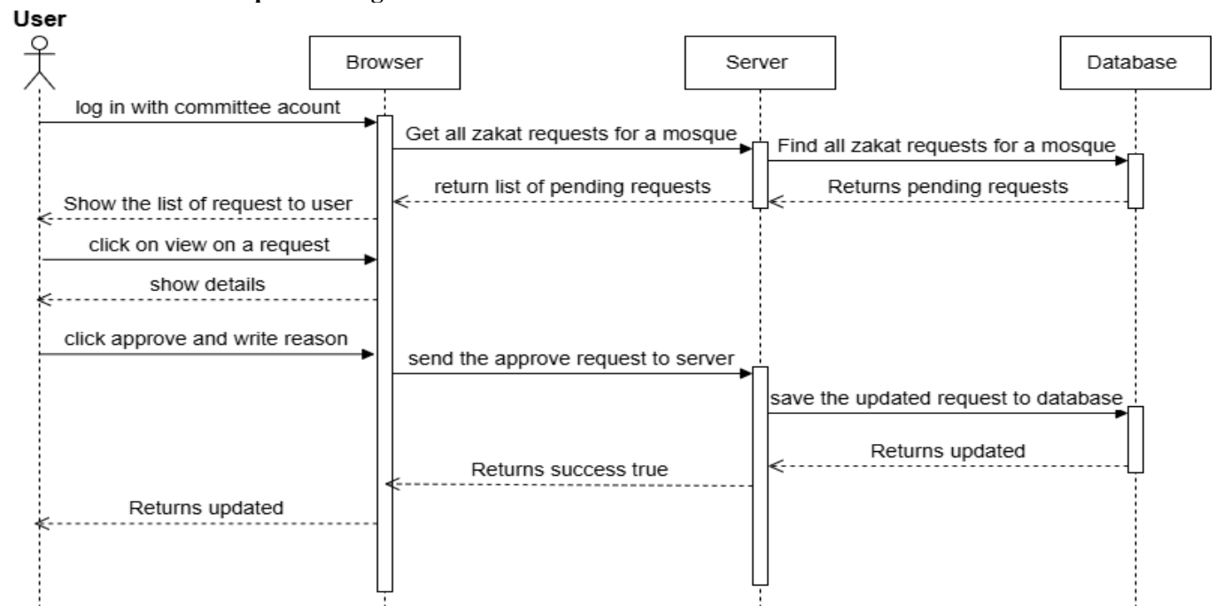
Figure 16 Committee review sequence diagram
