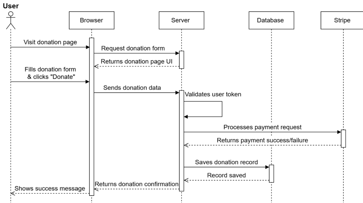
Figure 12 Online Donation Sequence Diagram
