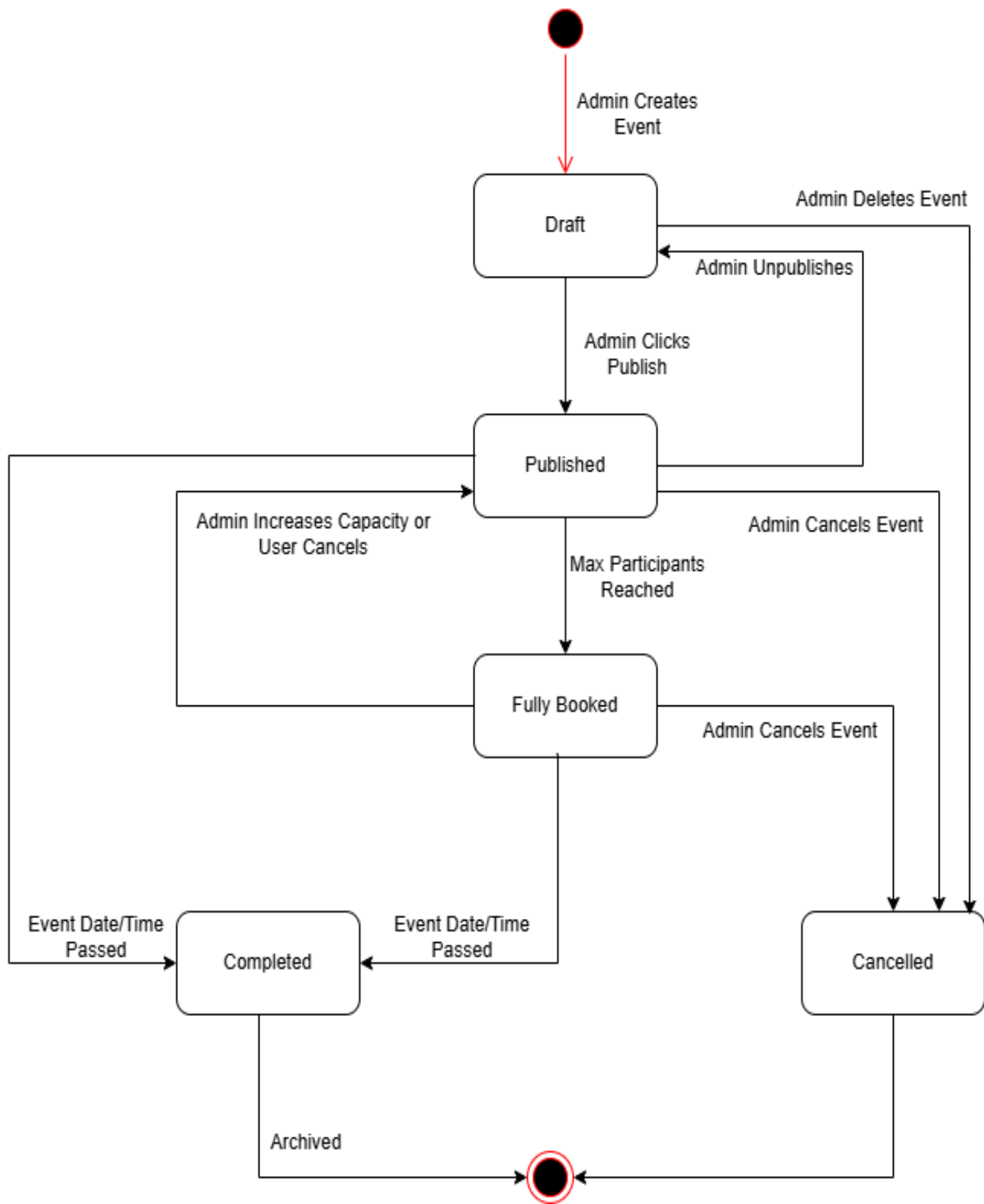
Figure 19 Event State Diagram
