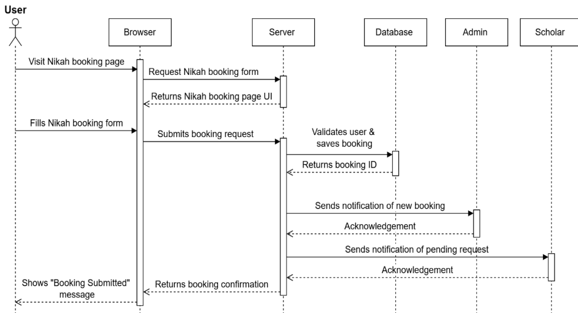
Figure 13 Nikah Booking Sequence Diagram
