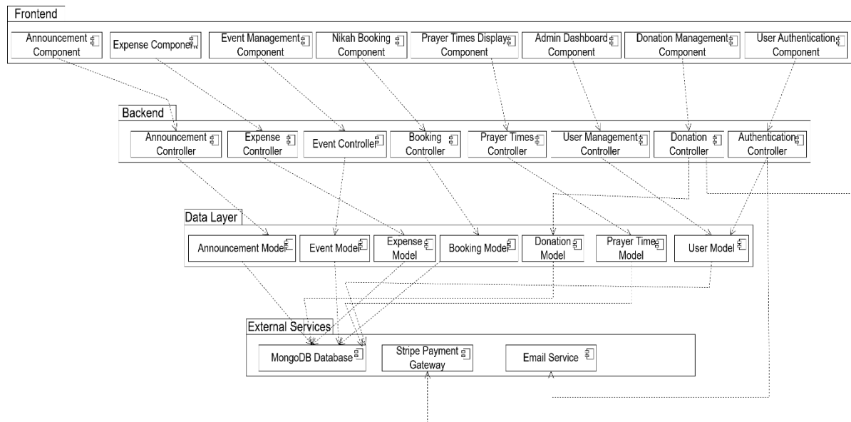
Figure 21 Component diagram
