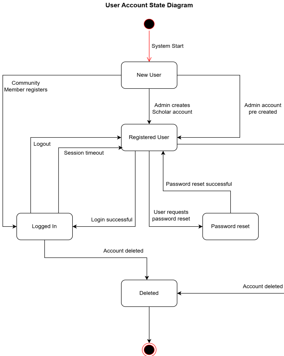
Figure 17 User Account State Diagram
