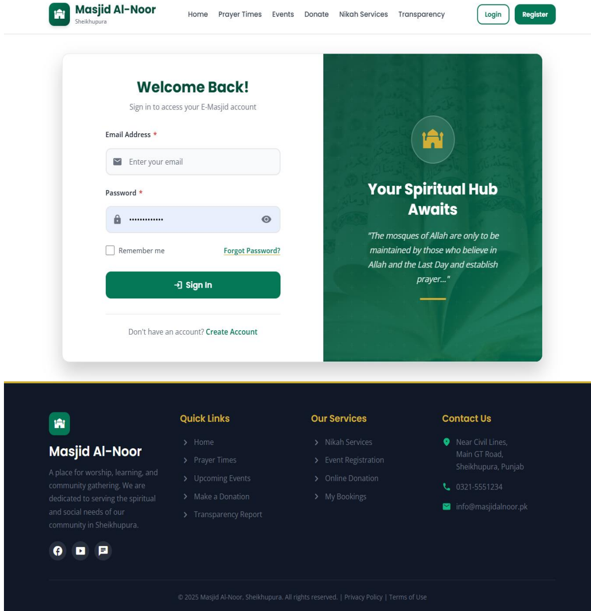
Figure 23 Login page design
