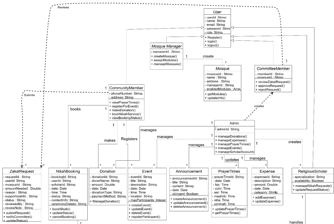
Figure 10 Class diagram
