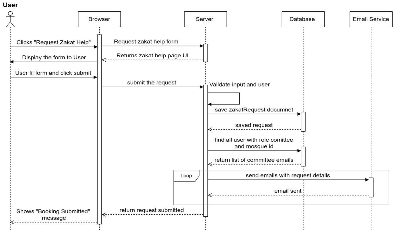
Figure 15 zakat request sequence diagram
