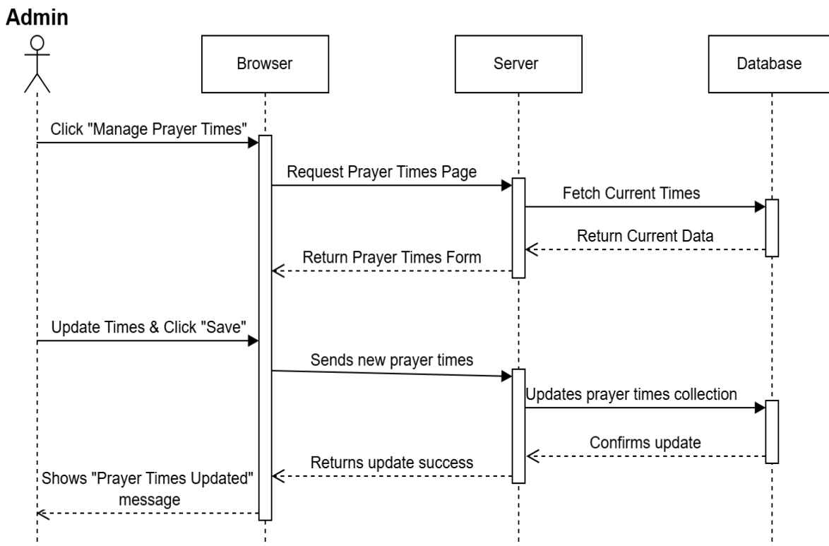
Figure 14 Admin Update Prayer Times Sequence Diagram
